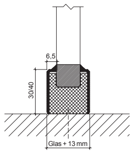
Floor connection
