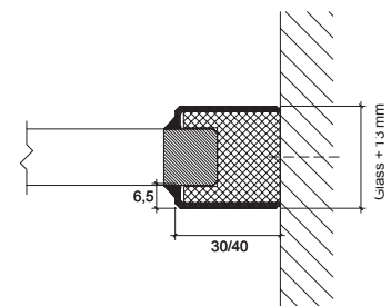
Wall connection
